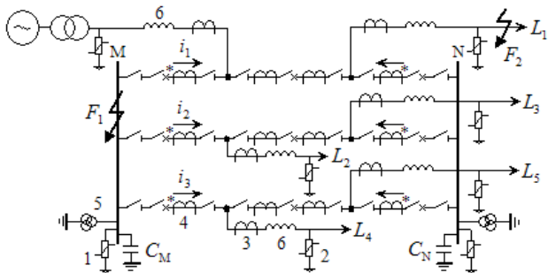
1— Bus MOA, 2— Line MOA, 3— CT of line protection, 4— CT of bus protection, 5— PT, 6— Wave trapper
