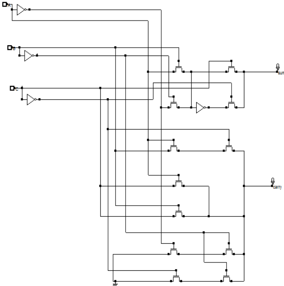
Figure 3. Proposed adder cell
