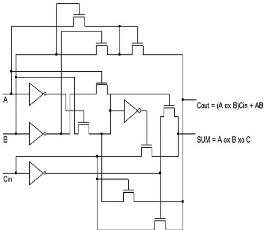
Figure 2.Full Adder
