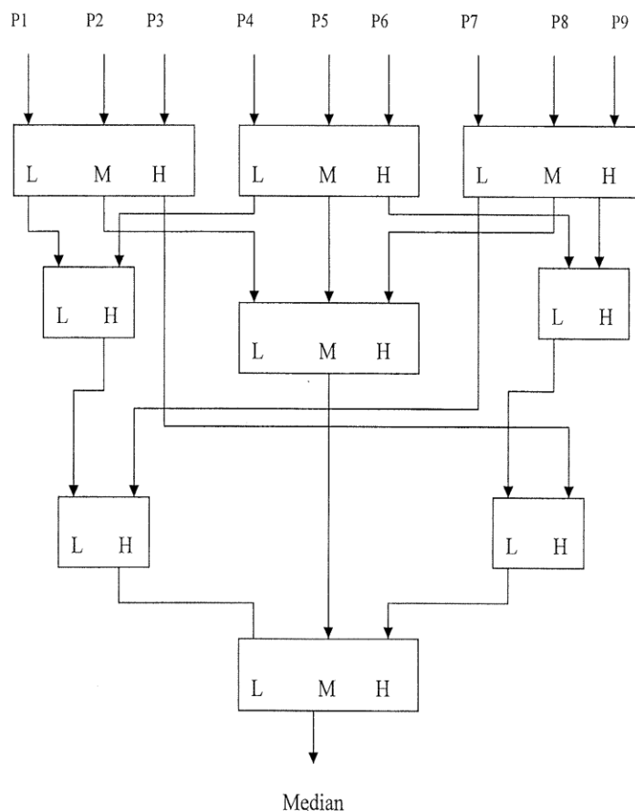
Figure 5. Block diagram of the sorter to find the median
