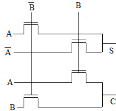
Figure.1 Half adder
