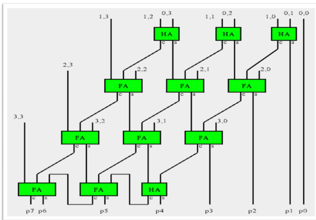
Figure 4. Carry save Array (CSA) Multiplier
