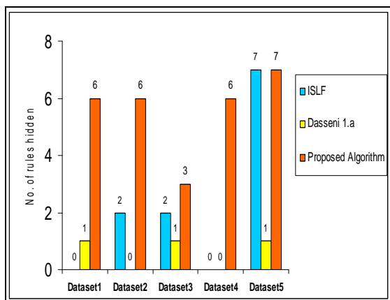
Figure 1: Performance Evaluation and Comparison of Existing and Proposed Algorithm
