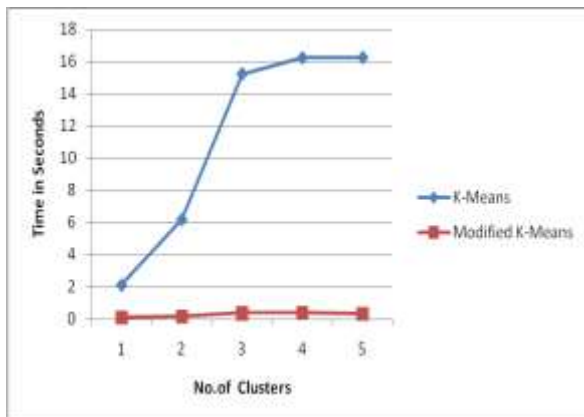
Fig.2. An Image Showing Time Complexity Analysis of H And G Indices Data
