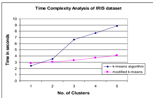
Fig.1. An Image Showing Time Complexity Analysis of Iris Dataset
