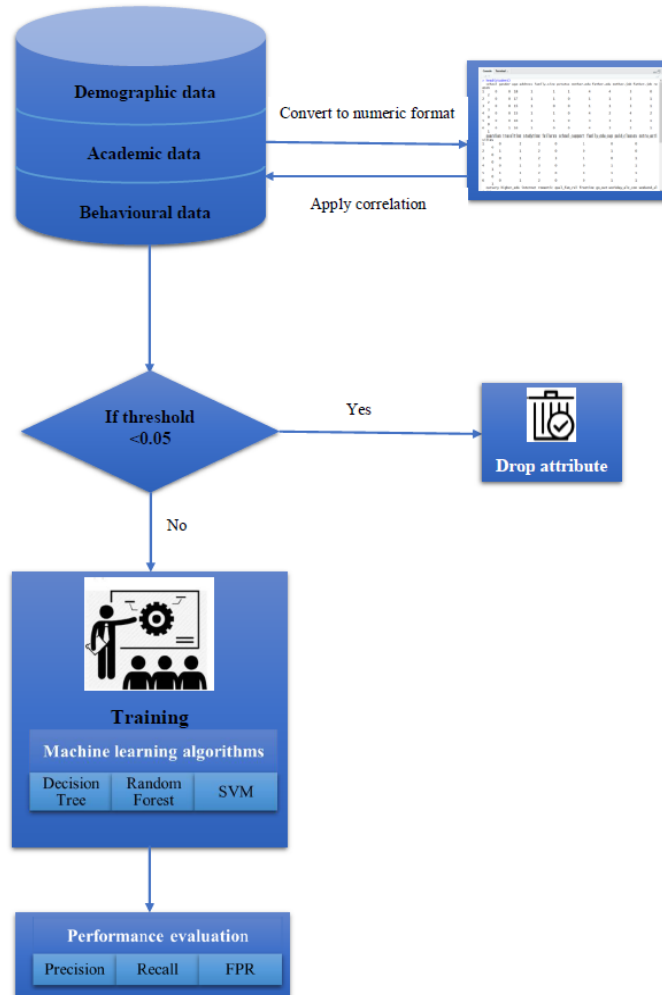
Fig. 1. Proposed methodology for student performance prediction
