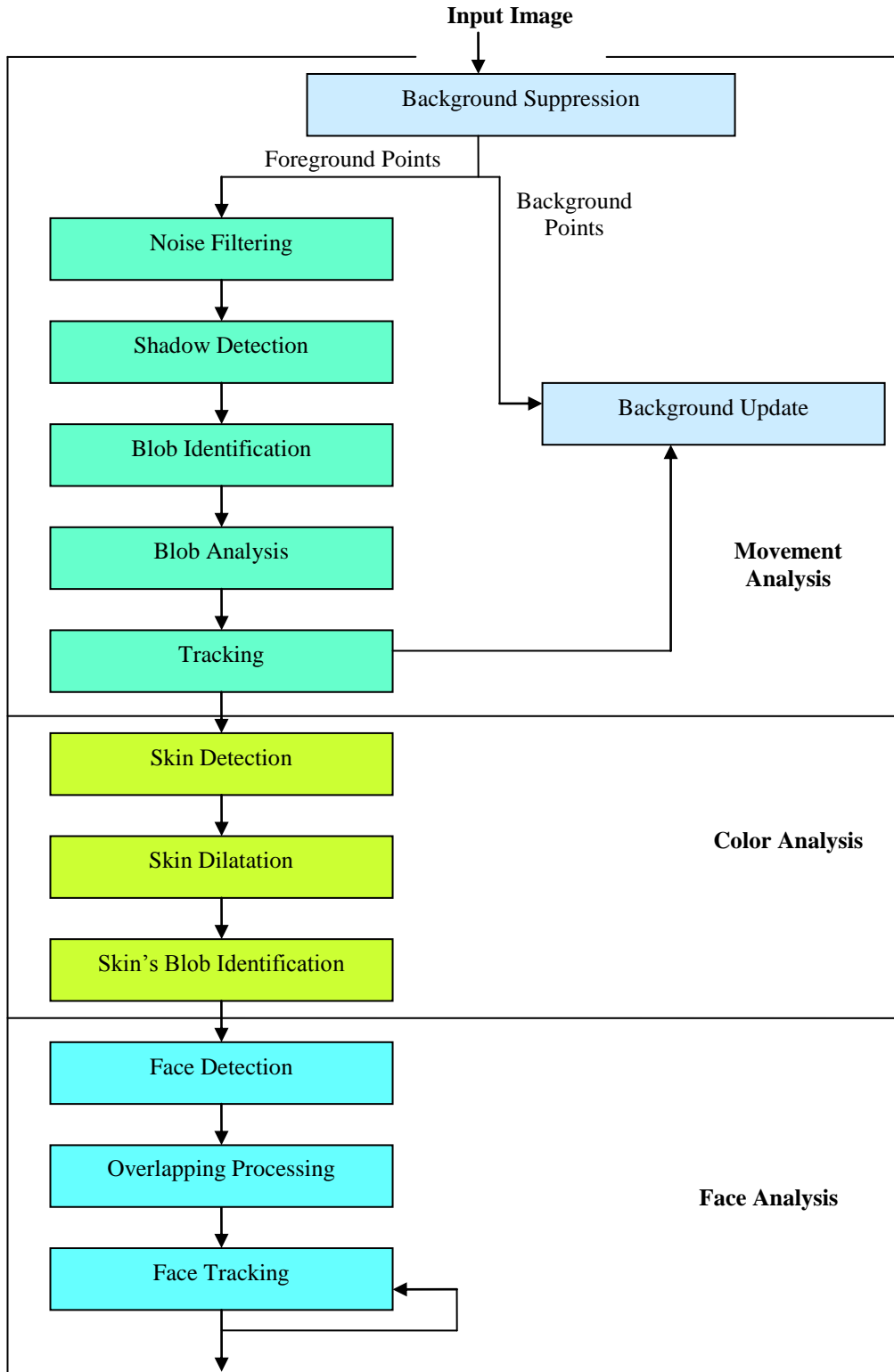
Fig. 1: Block Diagram of the Real Time Tracking of Multiple Human Faces Identification
